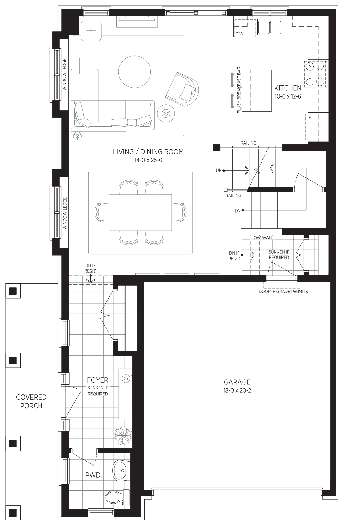
MAIN FLOOR PLAN 'A'
