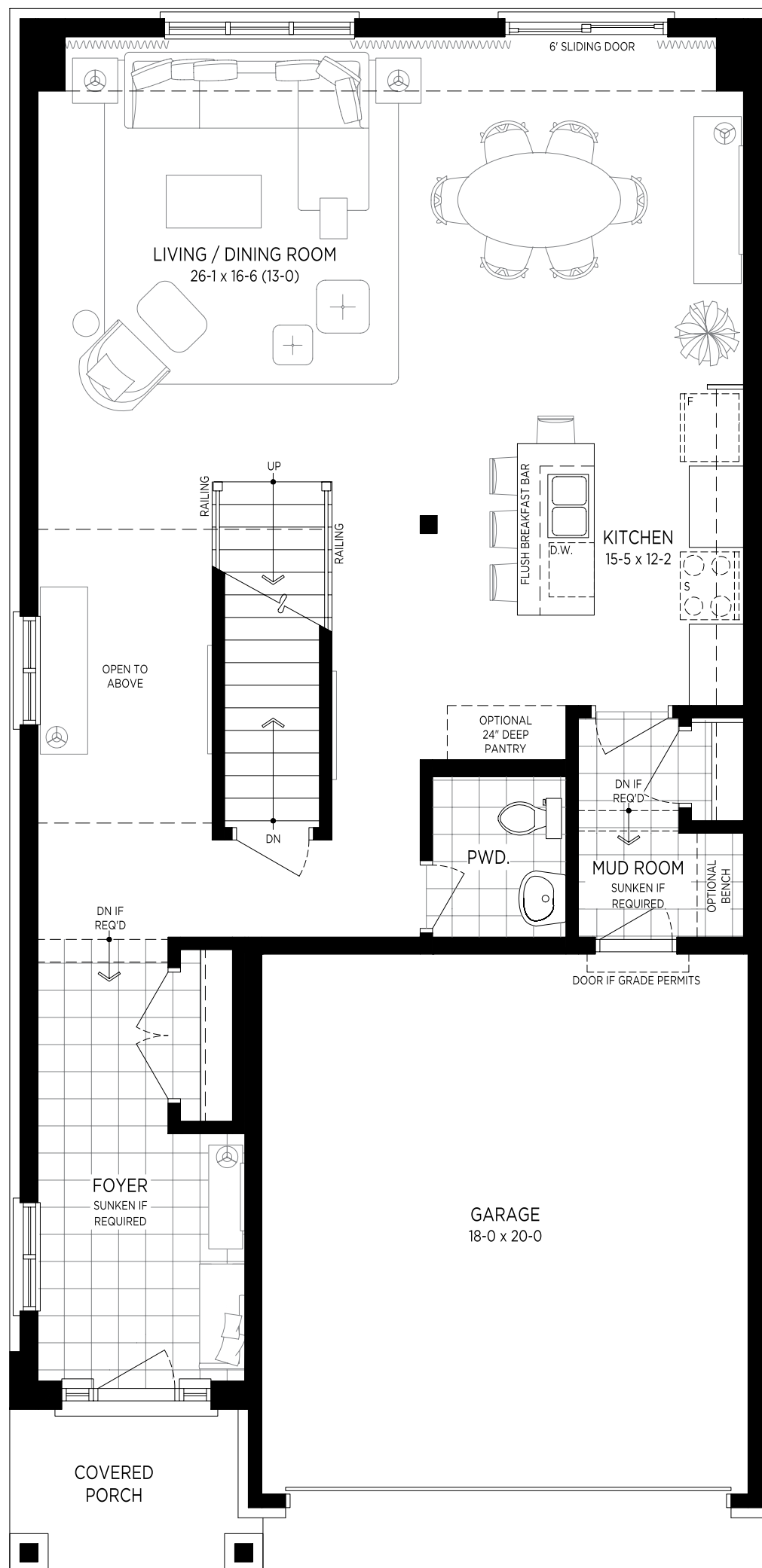
MAIN FLOOR PLAN 'A'
