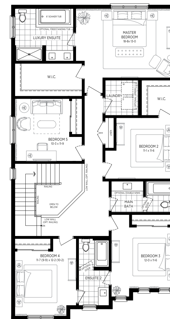
OPT. 3 - SECOND FLOOR PLAN 'A' 5 BEDROOM PLAN W/LUXURY ENSUITE
