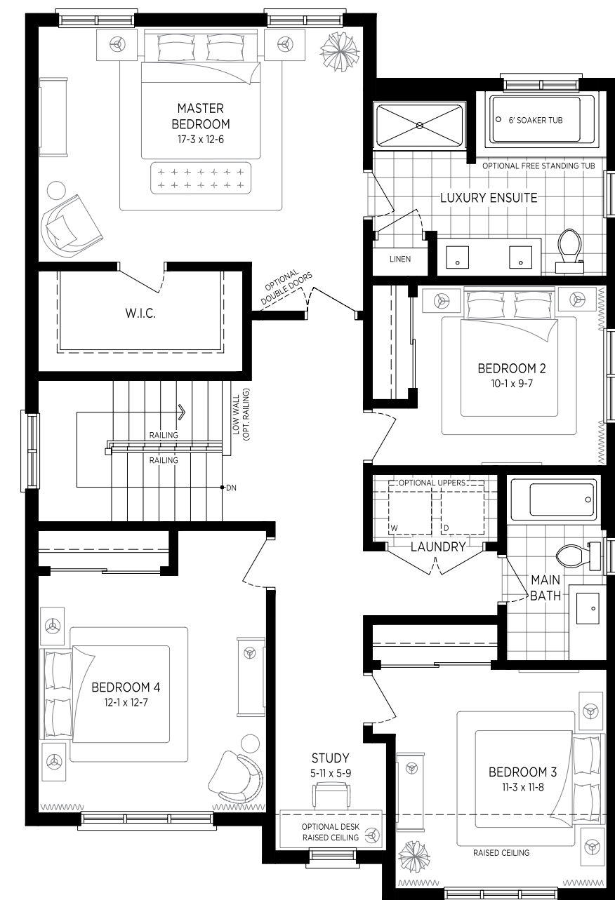
OPT. SECOND FLOOR PLAN 'A' 4 BEDROOM PLAN W/LUXURY ENSUITE
